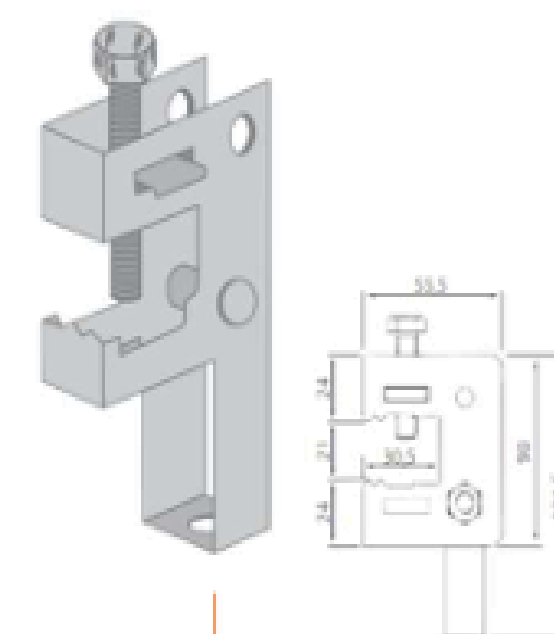
GRAMPO "C" BALANCIM
